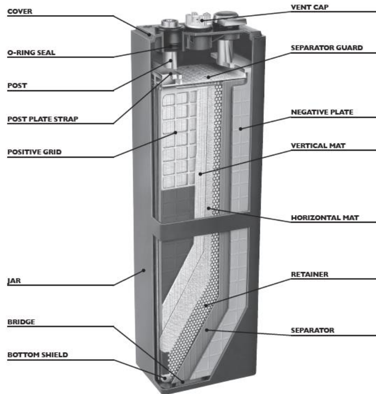
Figure 1 – conceptual design of an Industrial battery with descriptions and explanations necessary for the understanding of the drawings and schemes and the operation of the battery.
